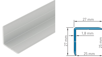
AP-200-025 L-Winkel Profil 25x25mm L-Bracket Profile 25x25mm
