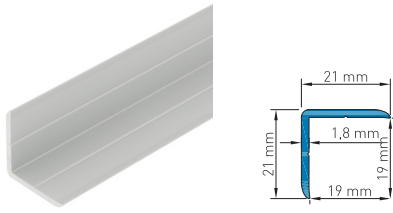
AP-200-019 L-Winkel Profil 19x19mm L-Bracket Profile 19x19mm
