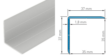
AP-200-035 L-Winkel Profil 35x35mm L-Bracket Profile 35x35mm
