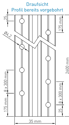
Top view Profile already pre-drilled
