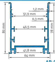
AP-003-006 Aluminium Profil SLO | Alu natur Aluminium profile SLO | natural aluminium
